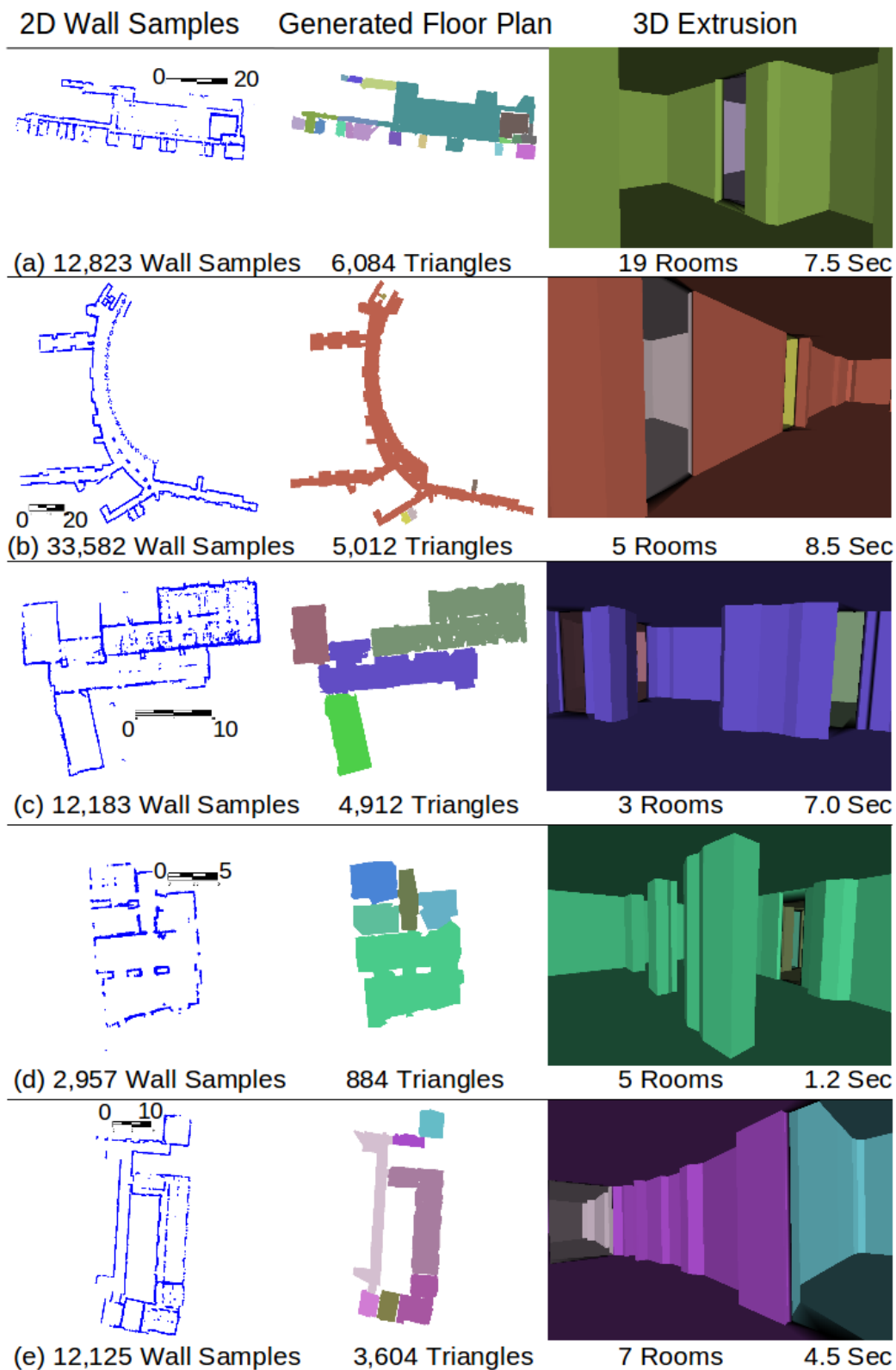
Figure 6: Example results of our approach. The left and middle columns show the input wall samples and the generated floor plan and room labeling, respectively. The right column shows a view of the interior of the extruded 3D model. Each row is labeled with the number of input samples, output triangles and rooms, as well as the total processing time to generate the model from data acquisitions that took several minutes to perform.
